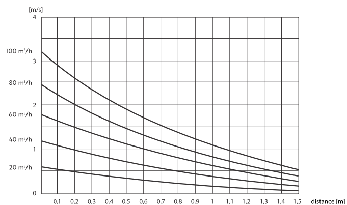
RONDO 100/125 velocity, m/s
